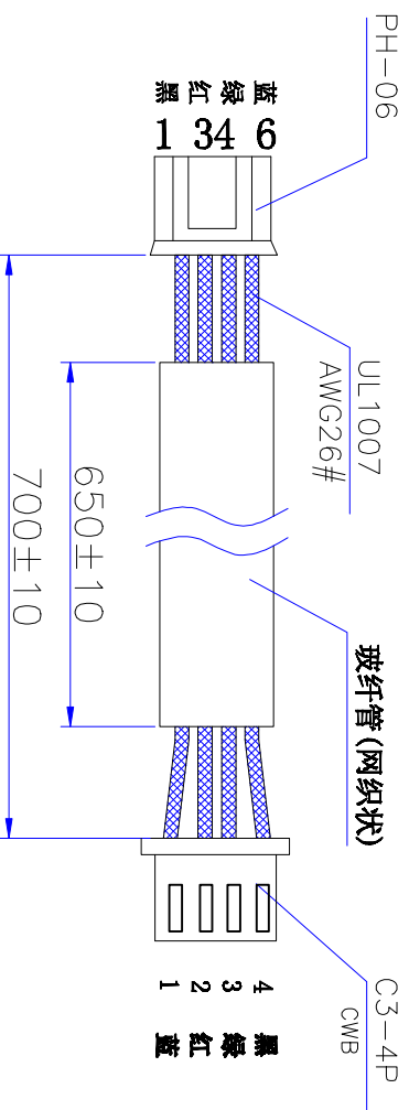
电气原理图 winding drawing
